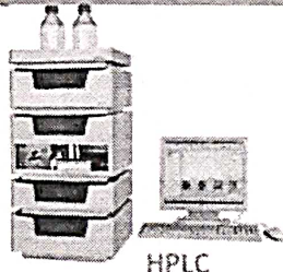
HPLC
